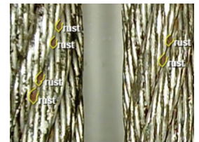
Cable Health Monitoring
